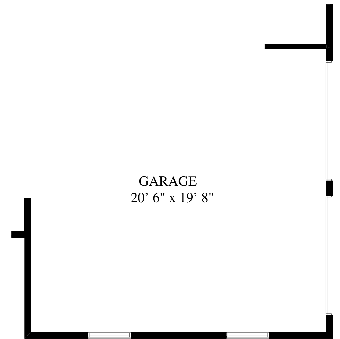
OPTIONAL SIDE ENTRY GARAGE
