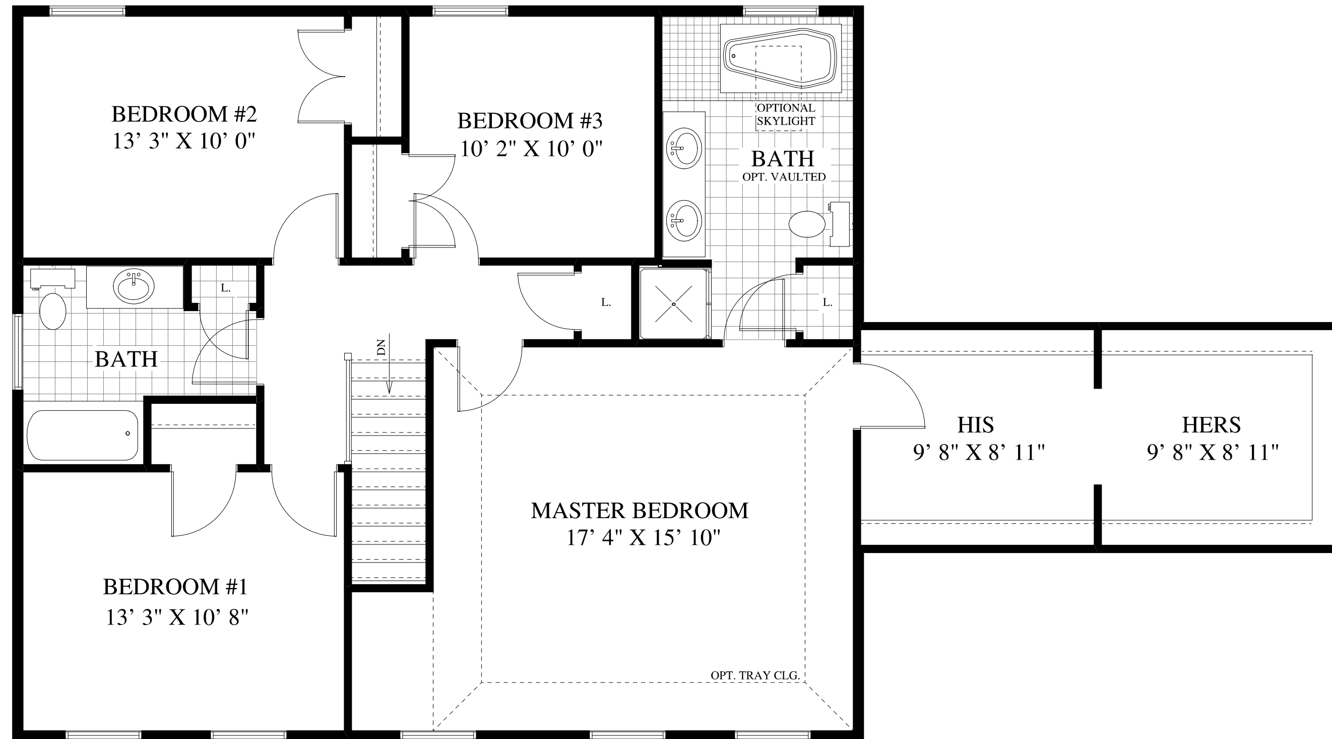
OPTIONAL SECOND FLOOR PLAN
