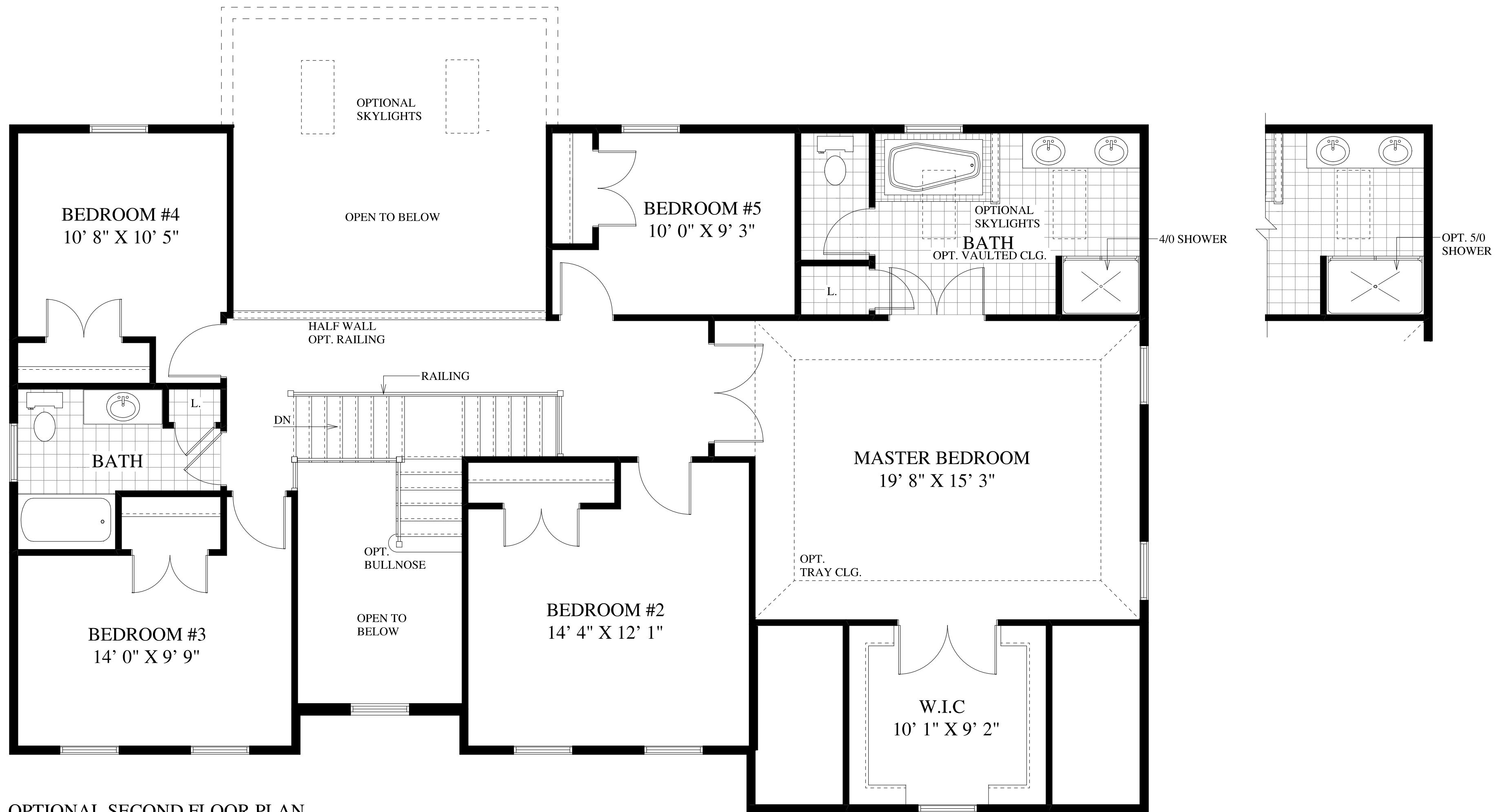
OPTIONAL SECOND FLOOR PLAN 5TH BEDROOM
